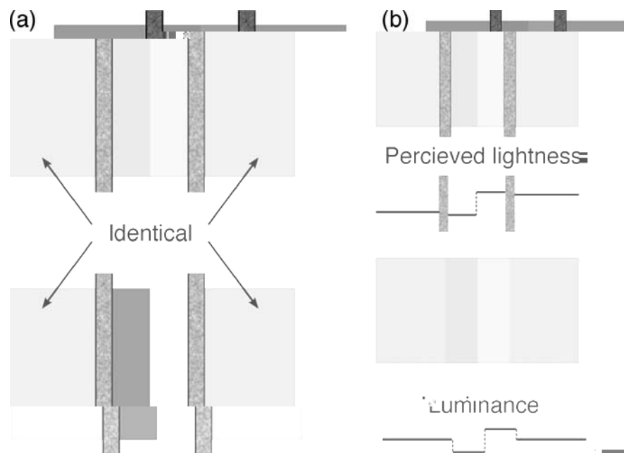
Figure 1. The “lightness effect”. (a) Perceptual grouping through amodal completion affects lightness. Physically identical flanking regions appear to differ in perceived lightness in the upper image: the left flank looks darker than the right flank. However, this lightness effect is not observed in the lower image (some observers even report a reversal of the effect, reminding us of the “simultaneous contrast” effect). This is presumably because of the breakdown of perceptual grouping due to the large luminance difference between the flanks and the central regions. (b) Perceived lightness and actual luminance along a horizontal cross-section.
